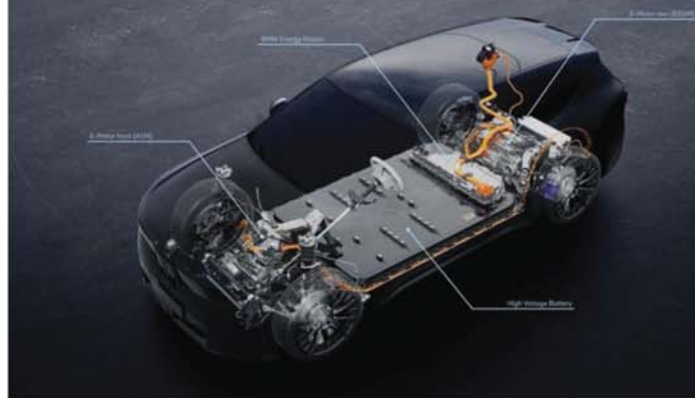
THE NEW BMW iX3 50 xDRIVE - POWERTRAIN.
