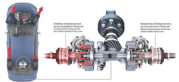
Audi S3 Limousine / Sedan Torque Splitter - Kraftverteilung Torque splitter - Power distribution 6x24
