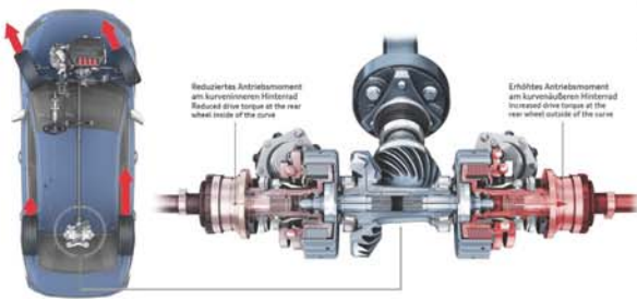
Audi S3 Limousine / Sedan Torque Splitter - Kraftverteilung Torque splitter - Power distribution 6x24
