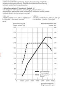
2,0 Liter-Vierzylinder-TFSI-Motor im Audi S3 2.0 liter four-cylinder TFSI engine in the Audi S3
