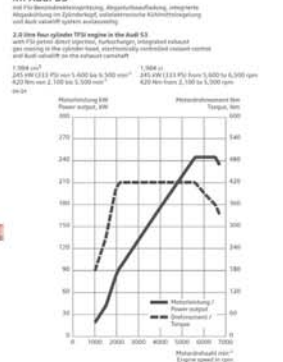
2,0 Liter-Vierzylinder-TFSI-Motor im Audi S3 2.0 liter four-cylinder TFSI engine in the Audi S3 6x24
